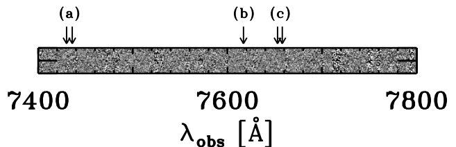
FIG. 3.— Two-dimensional spectrum of GN-108036 in the wavelength range of 7400 - 7800\text{\AA} . The size along the spatial axis is 5.0'' . No emission line is detected in this wavelength range, which argue against the possibility that the detected line at \simeq 9980\text{\AA} is \text{H}\alpha at z = 0.521 . In this case, an [\text{OIII}]\lambda 5007 line would have been detected at approximately 7617\text{\AA} marked by an arrow (b). No line detection also suggests that the detected line at \simeq 9980\text{\AA} is not either an [\text{OIII}]\lambda 5007 at z = 0.994 or \text{H}\beta at z = 1.054 . In the former/latter case, the [\text{OII}]\lambda\lambda 3726, 3729 doublet would have been detected at the position marked by arrows (a)/(c).
