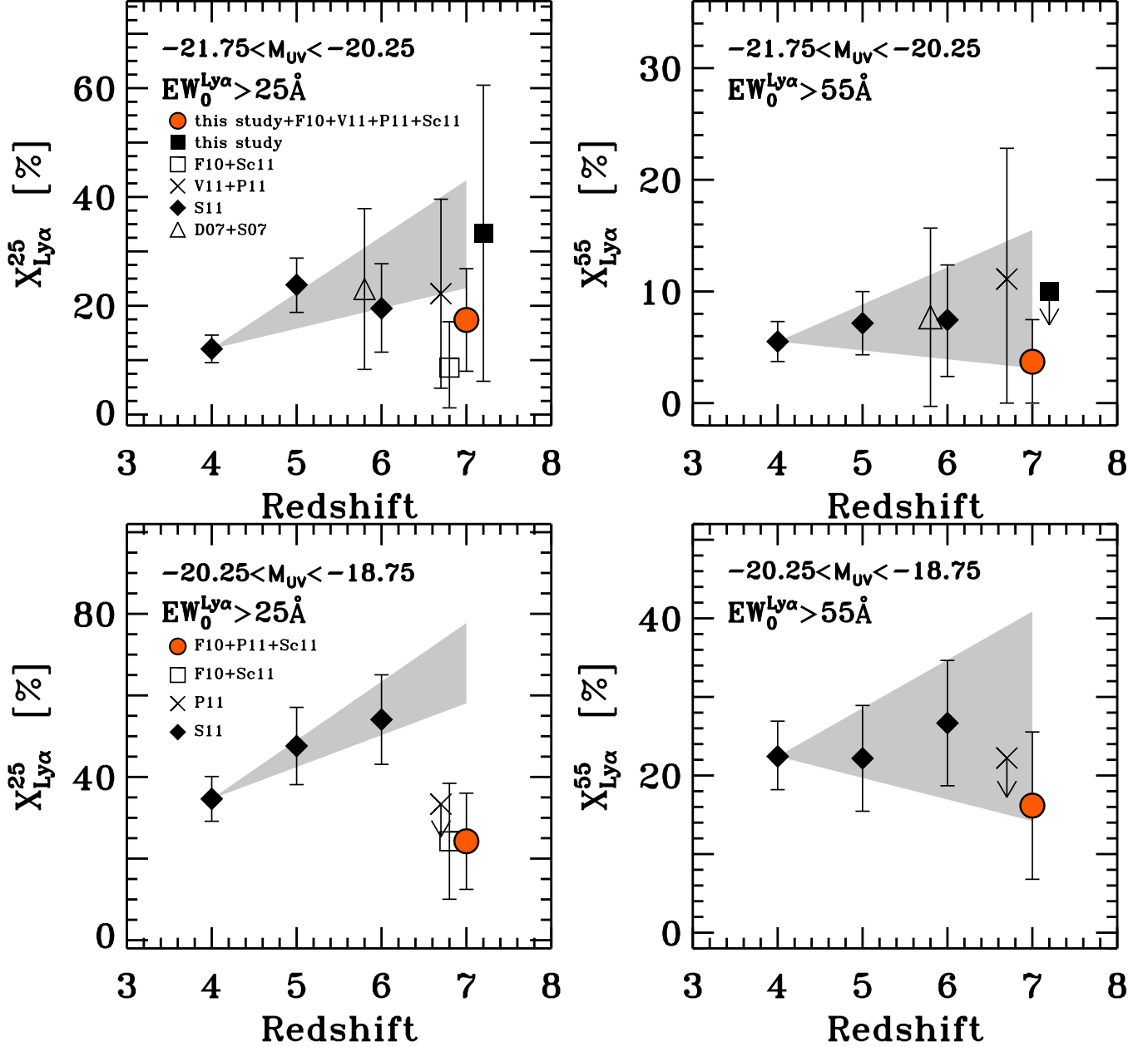
FIG. 8.— Evolution in the fraction of strong LAEs in LBGs with -21.75 < M_{\text{UV}} < -20.25 (top panels) and -20.25 < M_{\text{UV}} < -18.75 (bottom panels) over 4 < z < 7 . The left panels show the fraction of galaxies with EW larger than 25 \text{ \AA} , while the right panels show the fraction of those with EW larger than 55 \text{ \AA} . The filled square is our results, the open square is the results of Fontana et al. (2010) and Schenker et al. (2011), the cross is from Vanzella et al. (2011) and Pentericci et al. (2011), and the filled circle is the composite results. The filled diamonds are the results of Stark et al. (2011), and open triangle is the composite result of Dow-Hygelund et al. (2007) and Stanway et al. (2007). The filled square, open square, cross, and open triangle are shifted in redshift for clarity. The shaded area is derived by extrapolating the trend seen in lower redshifts to z \sim 7 (Stark et al. 2011).
